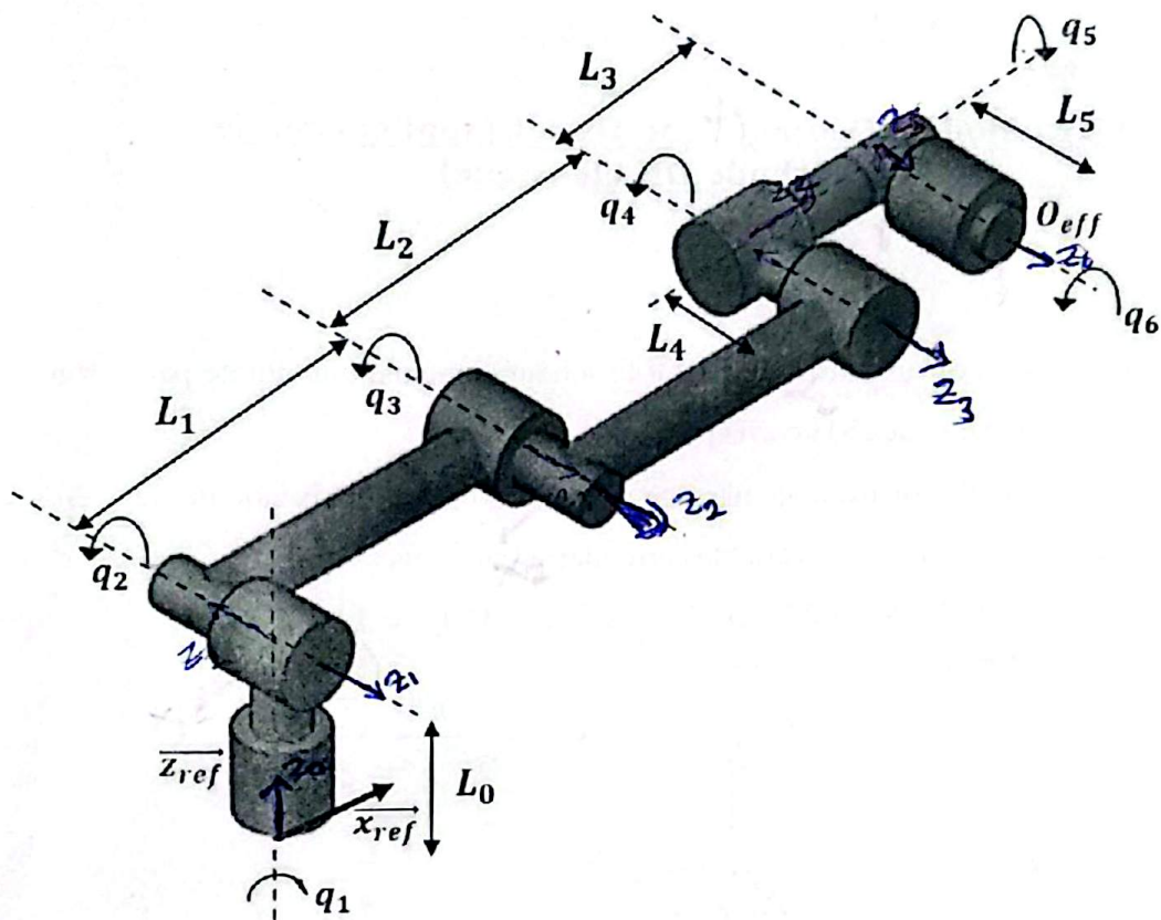
Figure 2 : Robot 6R
